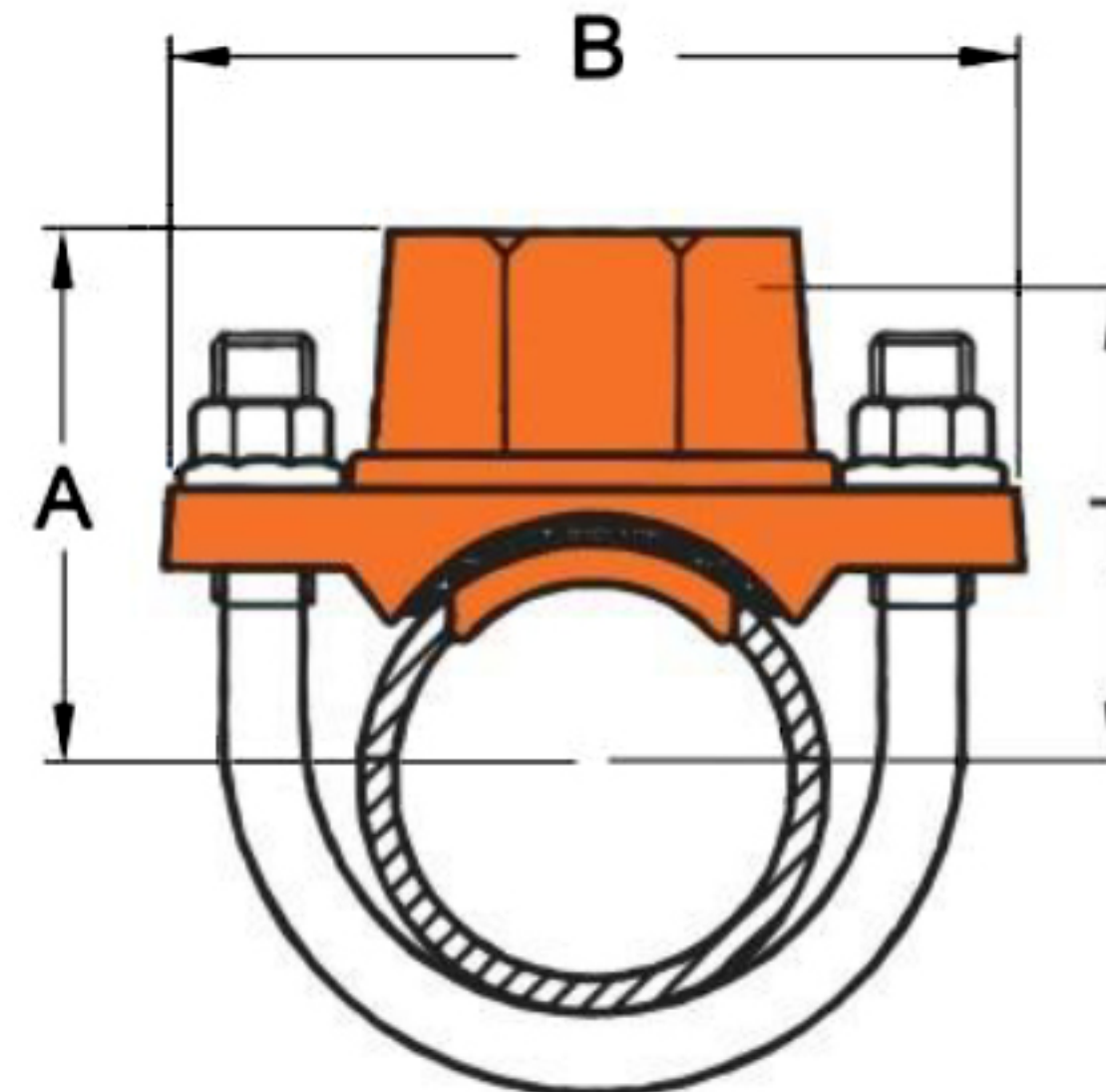
Model 723 “Saddle-Let” Small Mechanical Tee
